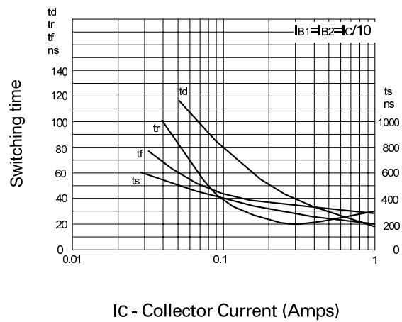
Switching Speeds
